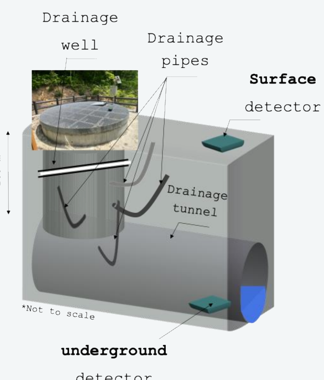
Conceptual deployment in existing drainage infrastructure ( Takisaka )
