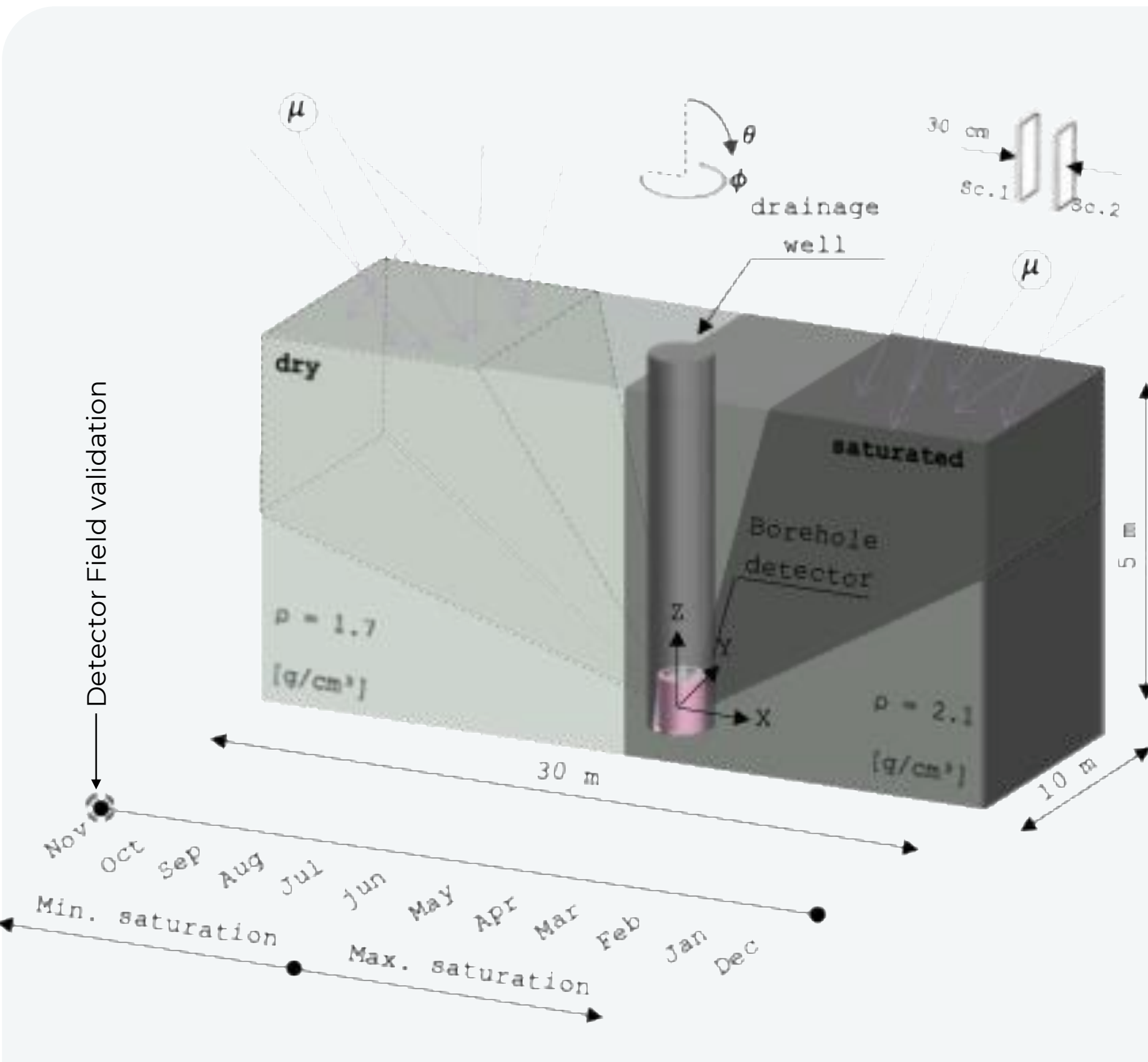
Schematic of target volume for dry/saturated contrast detection (idealized geometry)
