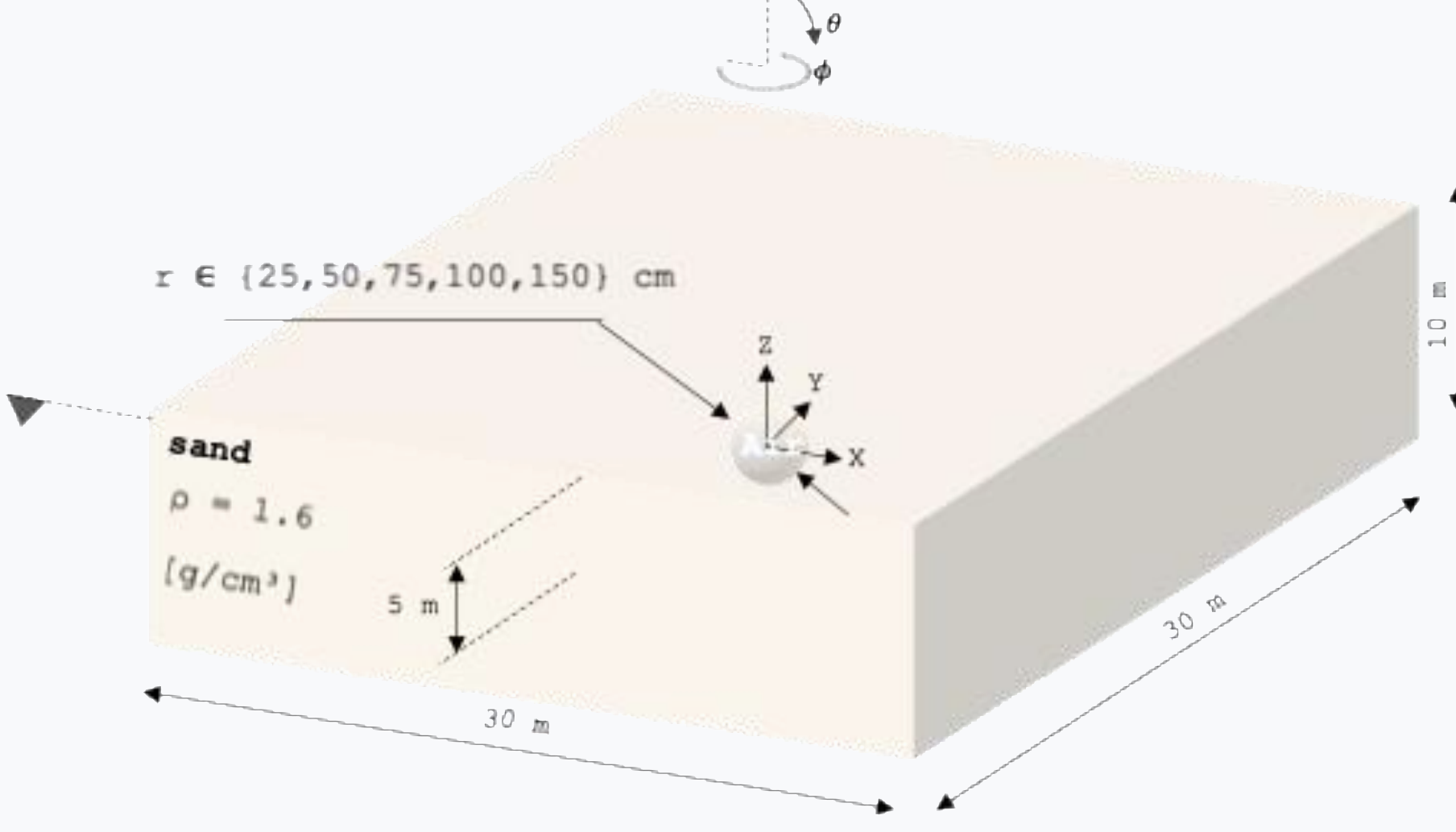
GEANT4 Simulation
