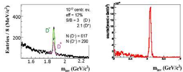
Fig. 10. Charm production in p+C collisions at 29 GeV: Open charm from D^+ + X , D^+ \rightarrow K\pi\pi (left) and charmonium from J/\psi + X , J/\psi \rightarrow \mu^+\mu^- (right).
