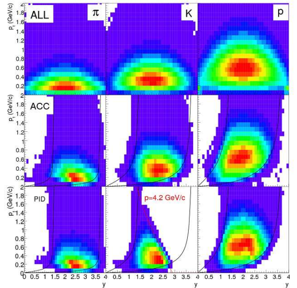
Fig. 6. Phase-space coverage of hadrons, produced in 25A GeV Au+Au collisions, in the CBM detector.
