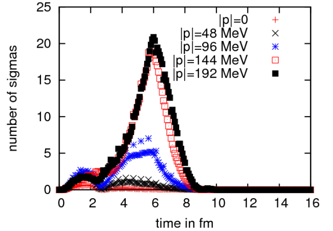
Fig. 3. Time evolution of the intensity of sigma fluctuations at a first order phase transition.
