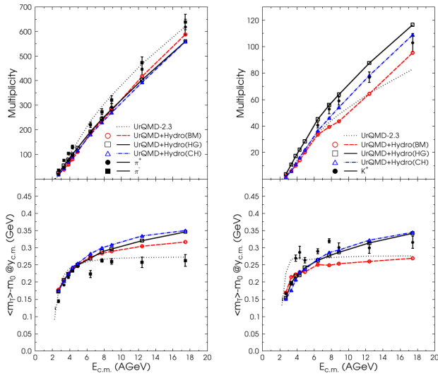
Fig. 1. Pion (left) and kaon (right) multiplicities (top) and mean transverse mass excitation function for central ( b < 3.4 fm) Au+Au/Pb+Pb collisions. The experimental data (full black symbols) are compared to hybrid model calculations with different equations of state (lines with symbols) and pure UrQMD 2.3 calculations (dashed line) [2, 5, 26–29]
