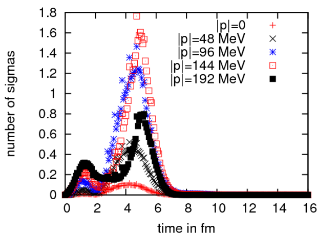
Fig. 4. Time evolution of the intensity of sigma fluctuations at a critical point.
