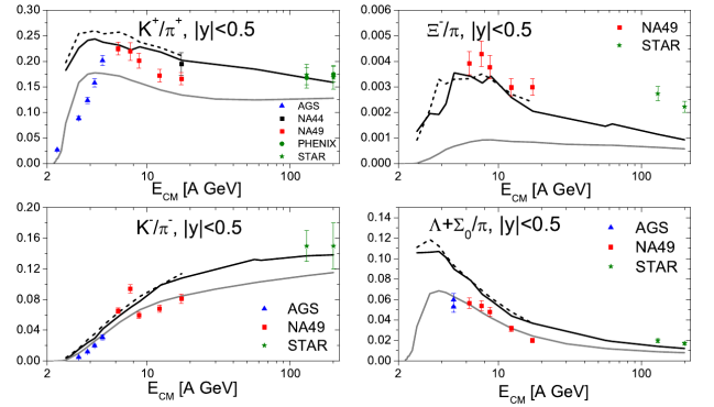
Fig. 2. Excitation function for kaon to pion ratios (left) and strange-baryon to pion ratios (right) for most central Au+Au/Pb+Pb collisions in the energy range \sqrt{s} = 2 - 200 A GeV. The hybrid model calculations are the solid and dashed black line for two different freeze-out criteria. UrQMD 2.3 results and experimental data [2, 5, 26–29] are shown for comparison.
